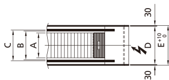
Detail Z
