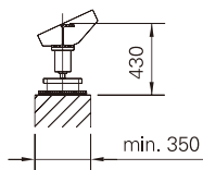
Detail X (1 intermediate support)
